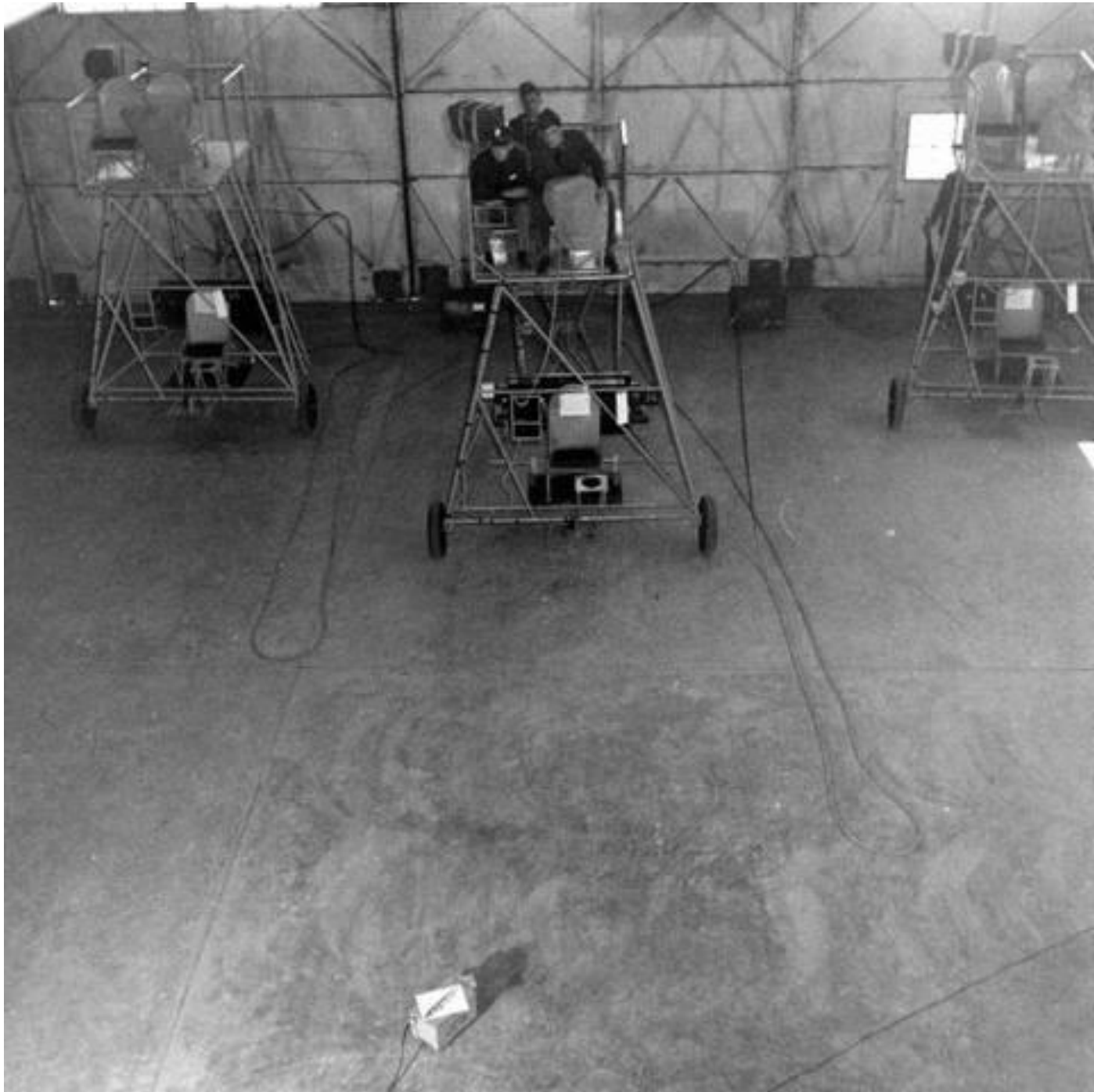
MOTORIZED BOMB SIGHT PLATFORM
